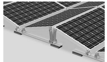
Flat roof east to west solar fixing
